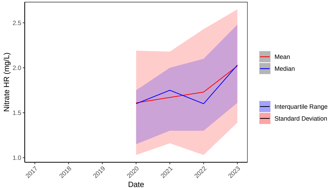
B2 Raceway 1 Nitrate HR (mg/L) Yearly Statistics
